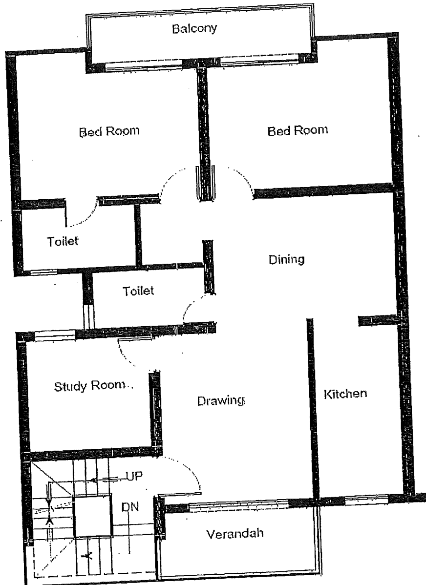
TYPICAL FLOOR PLAN BIG FLOOR PLAN
