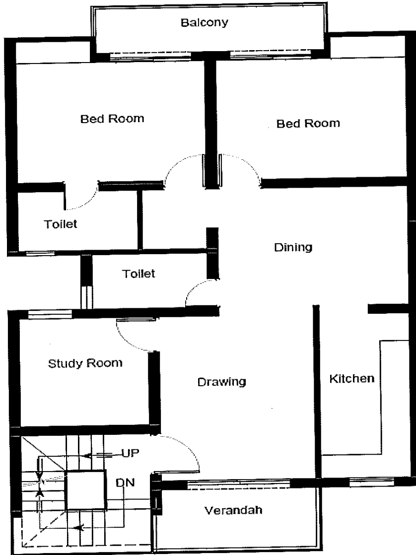
TYPICAL FLOOR PLAN FOR FIRST AND SECOND FLOOR
