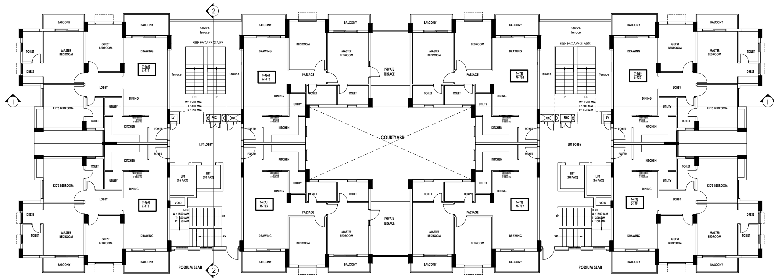
1ST FLOOR PLAN (TYPE-1A TOWER NO. - T-04)
