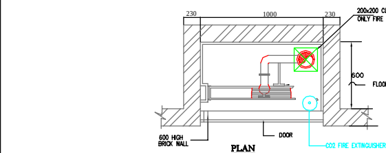
DRAWING: TYPICAL DETAIL FOR FIRE HOSE CABINET-1 SCALE=NTS [FHC-1]
