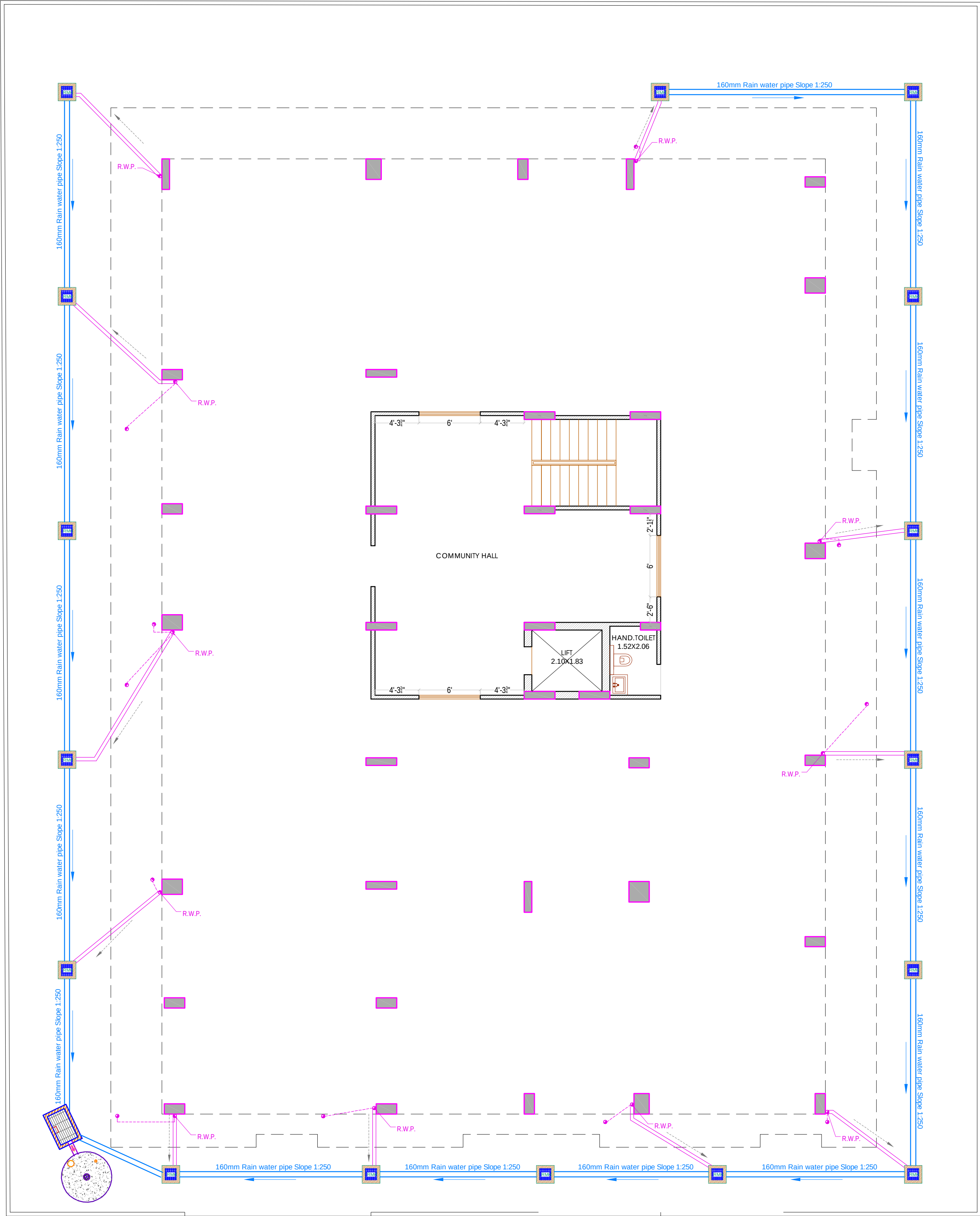
STILT FLOOR RAIN WATER HARVESTING LAYOUT PLAN
