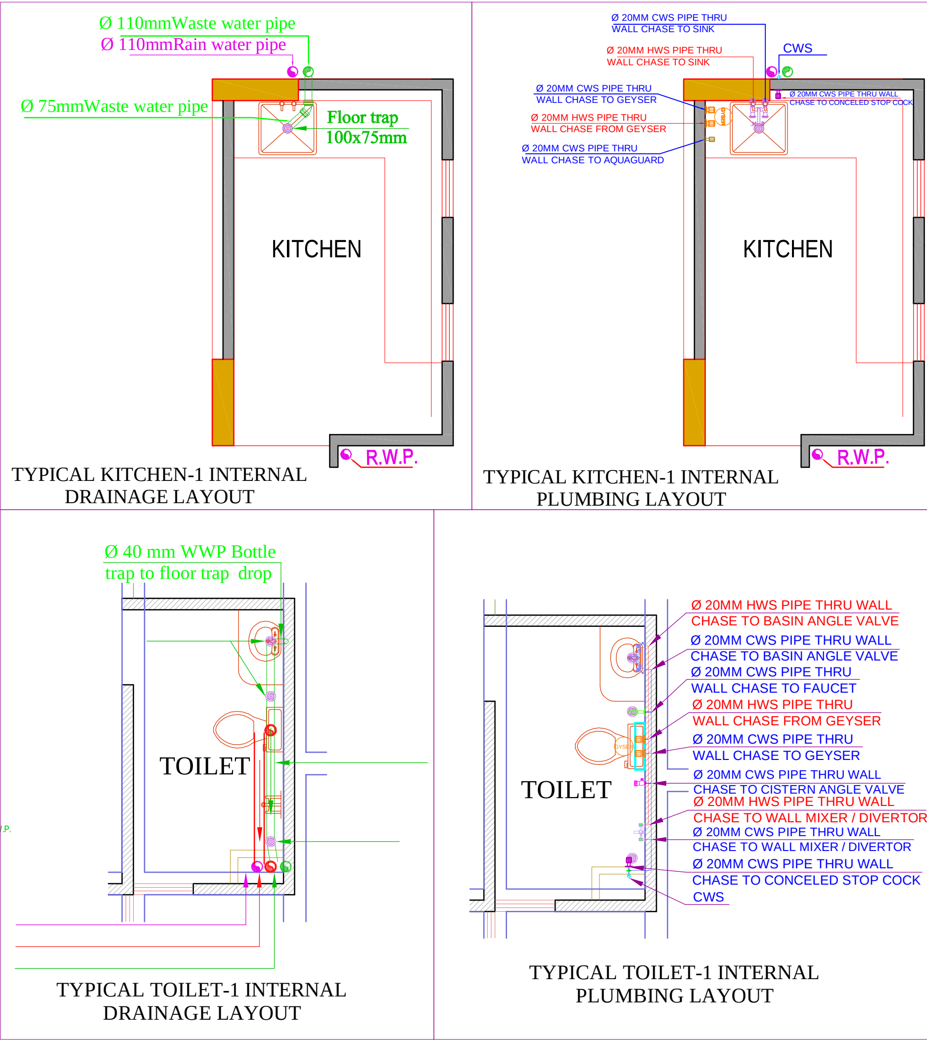
WATER SUPPLY DETAILS
