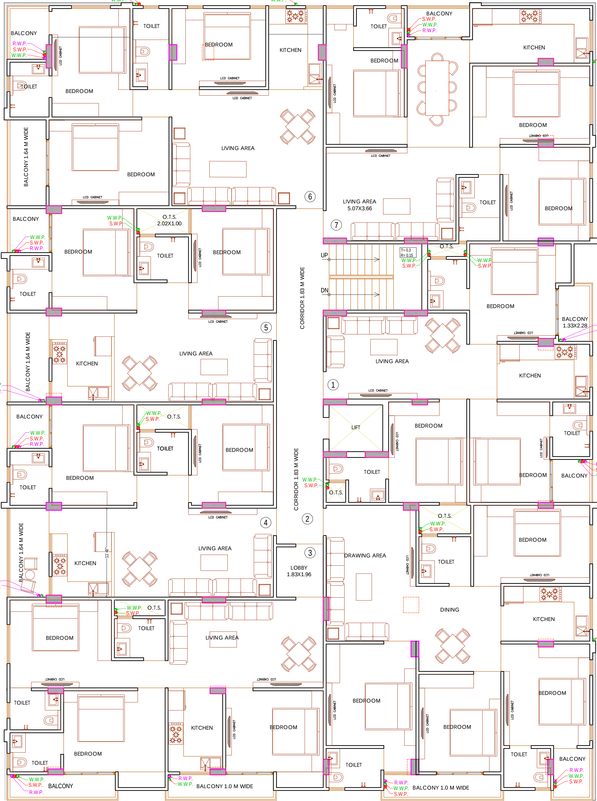
TYPICAL FLOOR SANITARY LAYOUT PLAN
