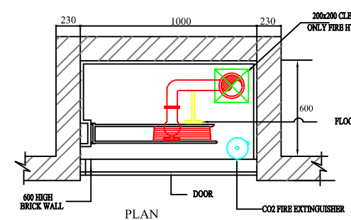
DRAWING: TYPICAL DETAIL FOR FIRE HOSE CABINET-1 SCALE: NTS [FHC-1]
