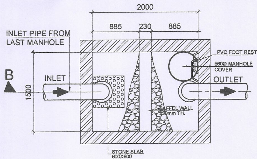
PLAN OF DESILTING CHAMBER & RWH PIT
