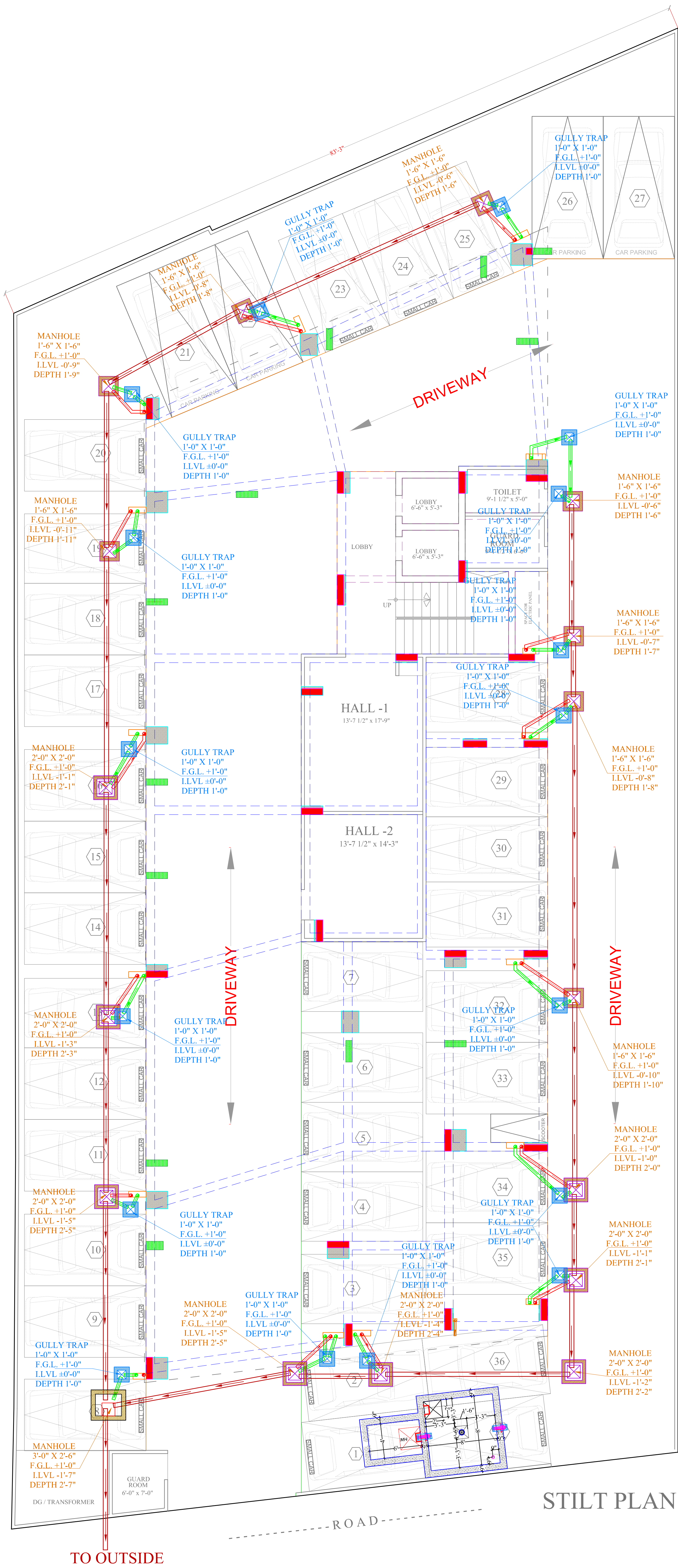
STILT FLOOR PLAN (PRACTICAL) PROPOSED CAR = 37
