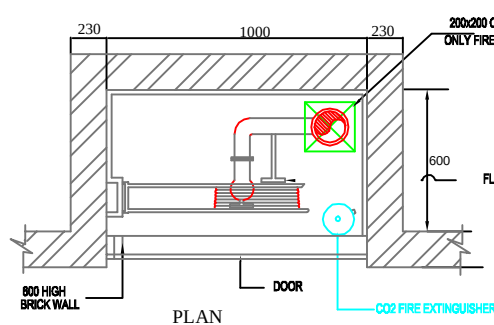
DRAWING: TYPICAL DETAIL FOR FIRE HOSE CABINET-1 SCALE:-N.T.S. FHC-1
