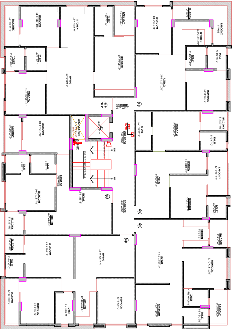
5th & 6TH FLOOR PLAN
