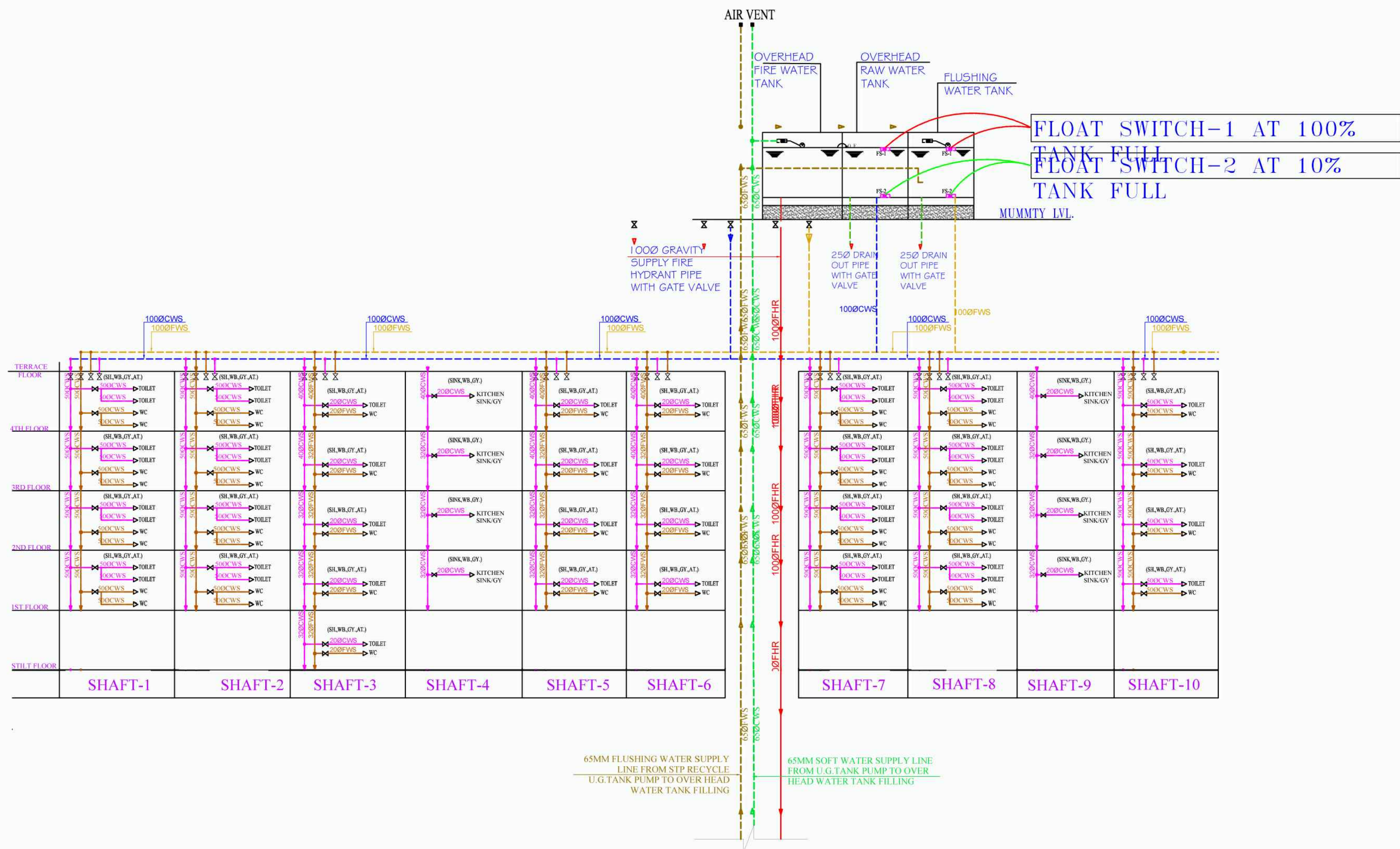
Water Supply Diagram
