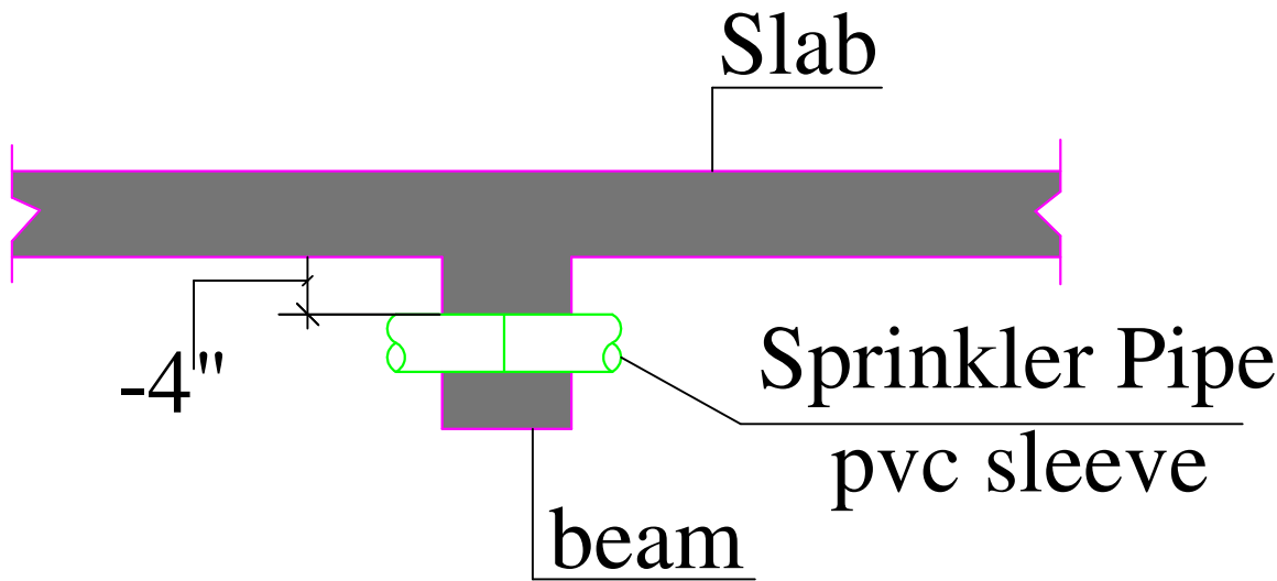
Typical Section of Sleeve in Beam for Sprinkler Pipe/ Lvl -4" below roof bottom
