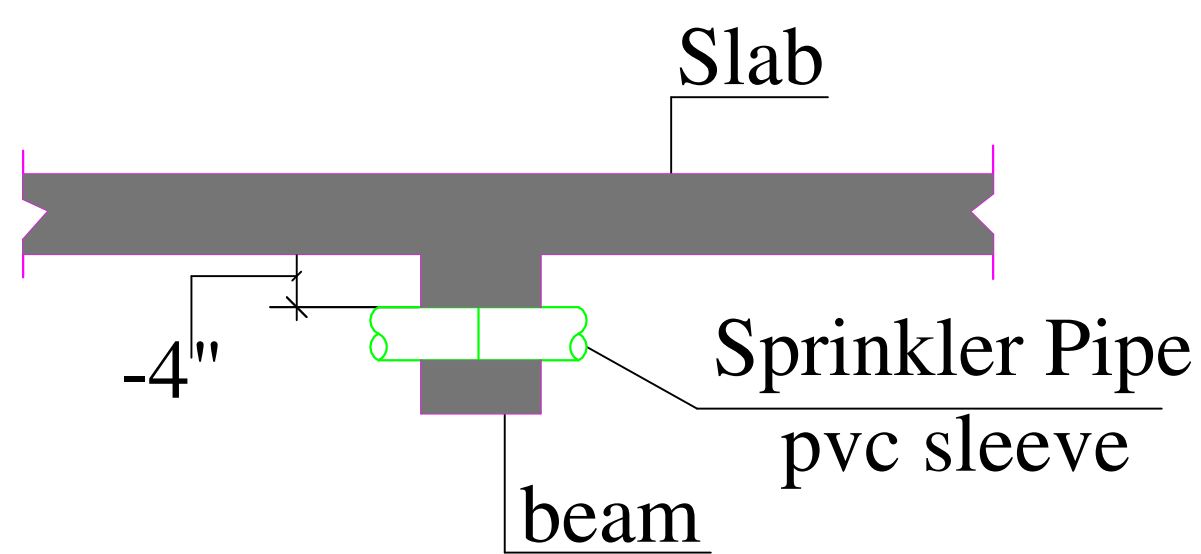
Typical Section of Sleeve in Beam for Sprinkler Pipe/ Lvl -4" below roof bottom
