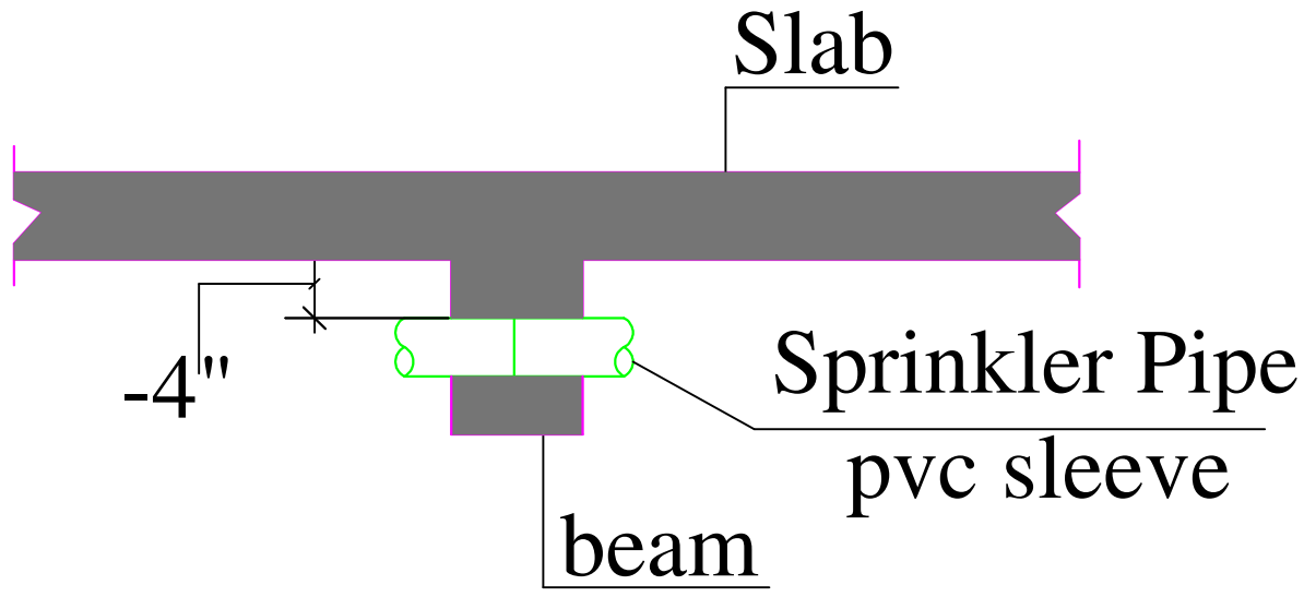
Typical Section of Sleeve in Beam for Sprinkler Pipe/ Lv1 -4" below roof bottom
