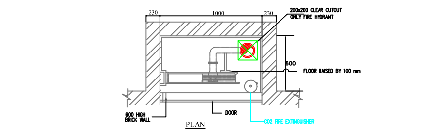
DRAWING: TYPICAL DETAIL FOR FIRE HOSE CABINET-1 SCALE: NTS [FHC-1]
