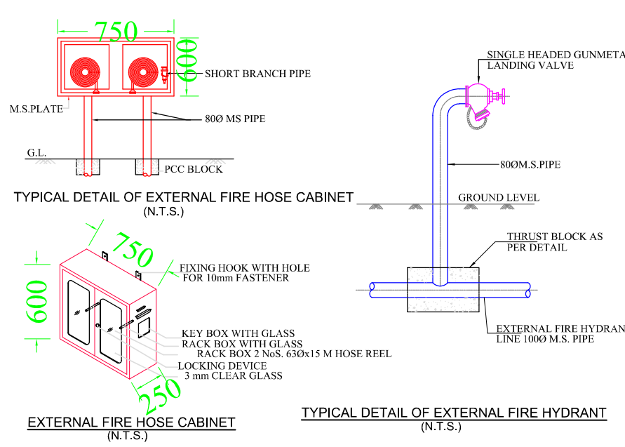
DRAWING: TYPICAL DETAIL FOR FIRE HOSE CABINET-1 SCALE: NTS [FHC-1]
