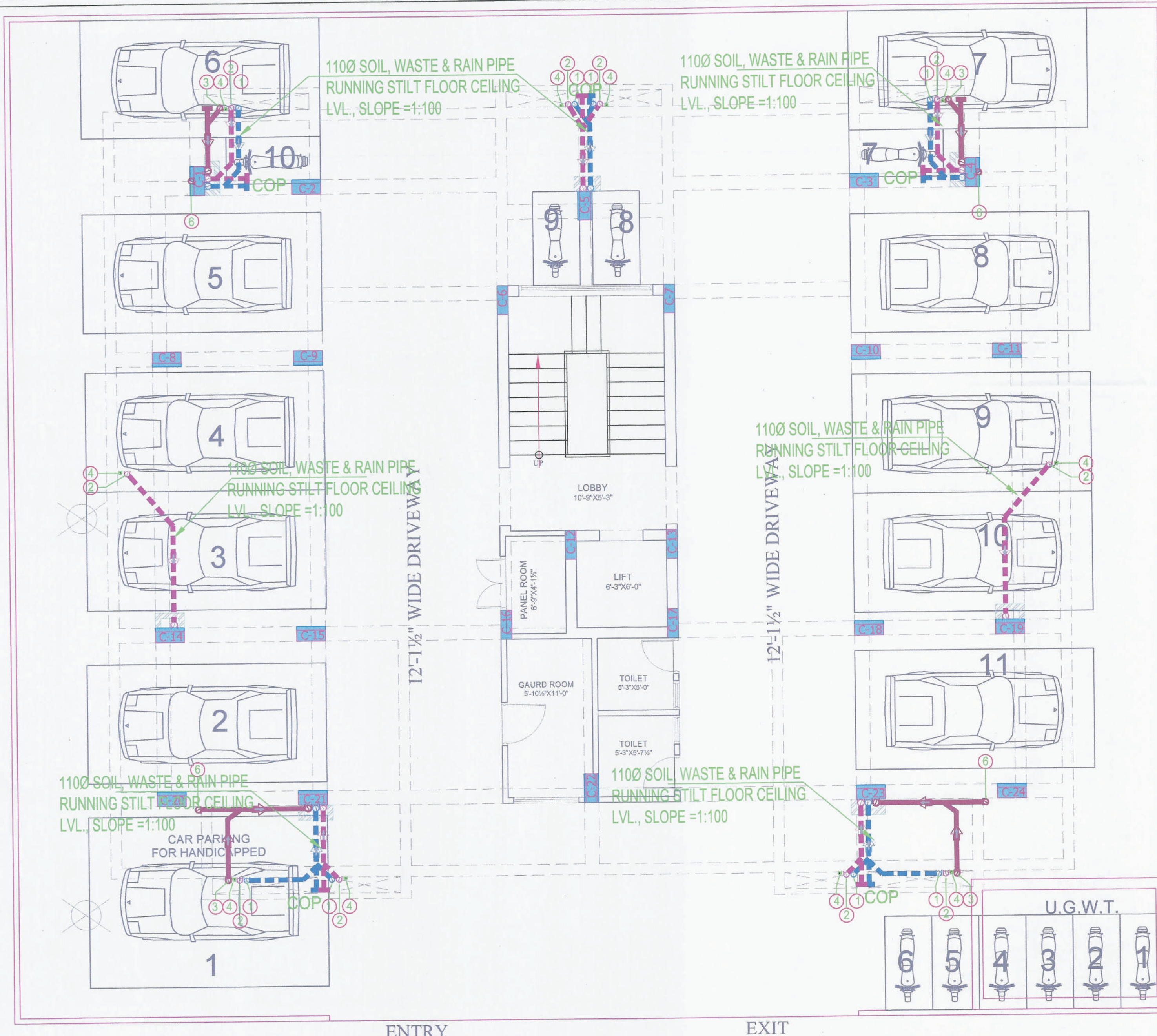
STILT FLOOR PLAN
