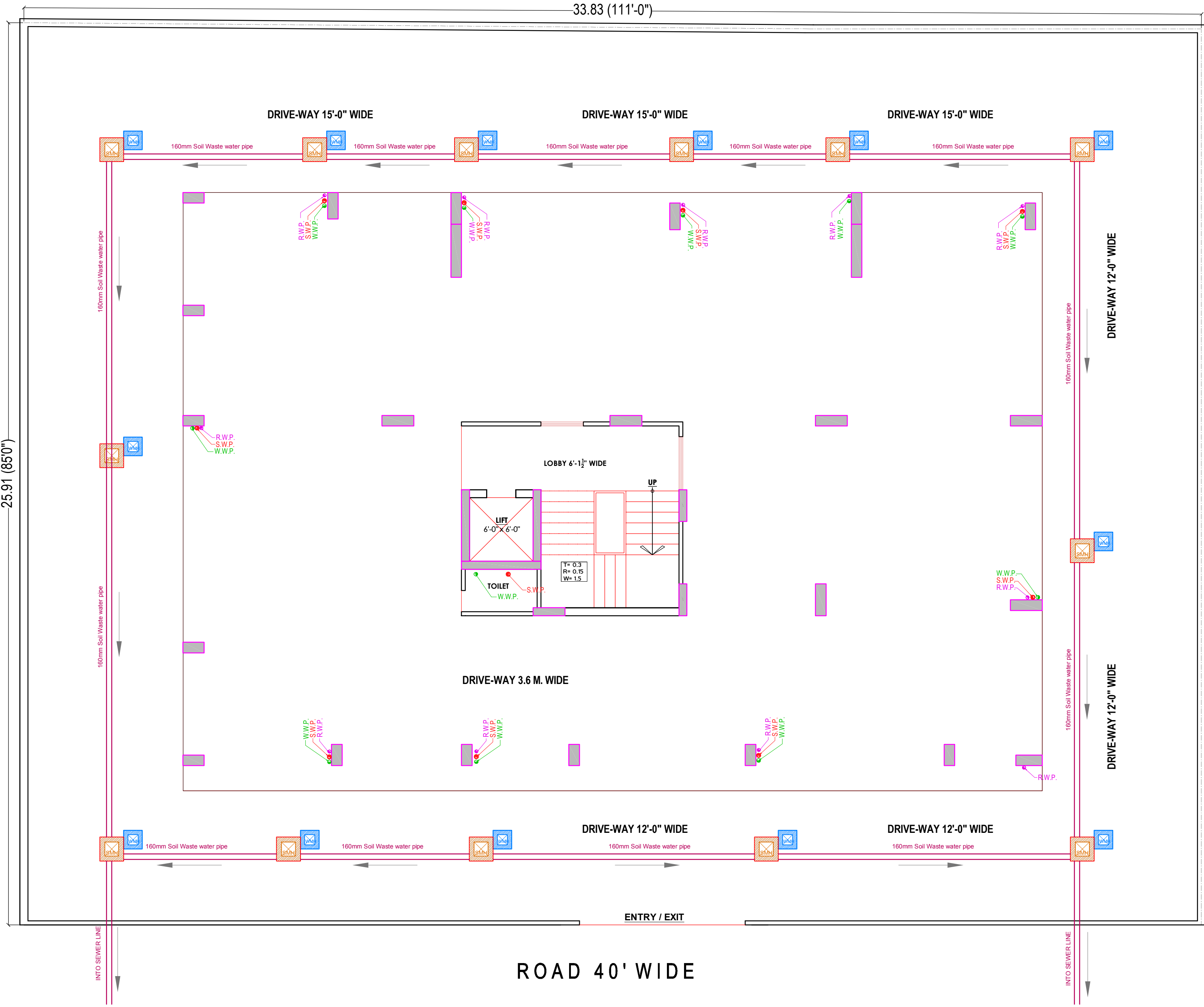
STORM WATER DRAINAGE & SOILD WATER DISPOSAL LAYOUT
