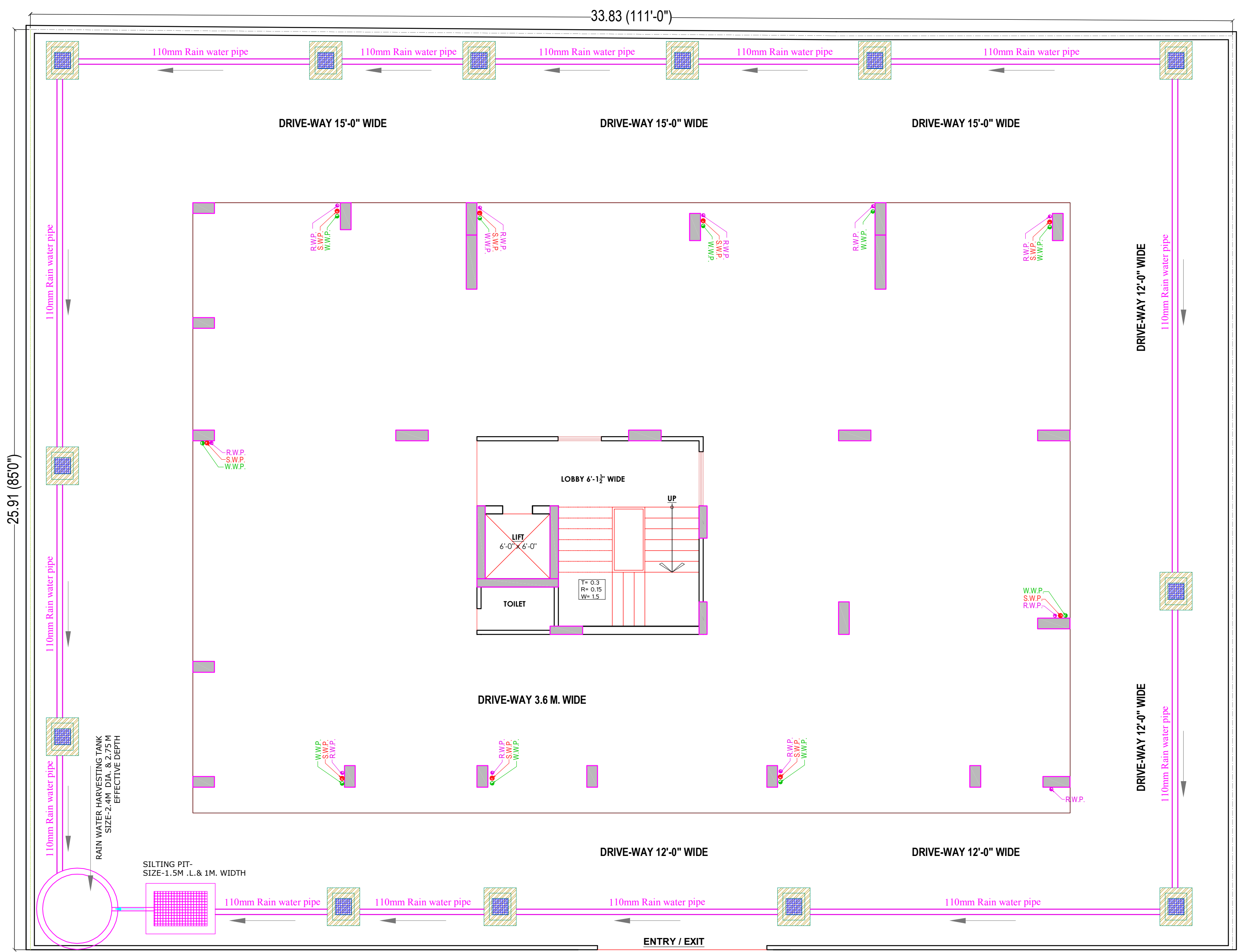
STILT FLOOR RAIN WATER HARVESTING LAYOUT PLAN
