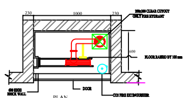
DRAWING: TYPICAL DETAIL FOR FIRE HOSE CABINET-1 SCALE: 1/4" = 1'-0"
