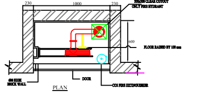
DRAWING: TYPICAL DETAIL FOR FIRE HOSE CABINET-I SCALE: 1/8" = 1'-0"
