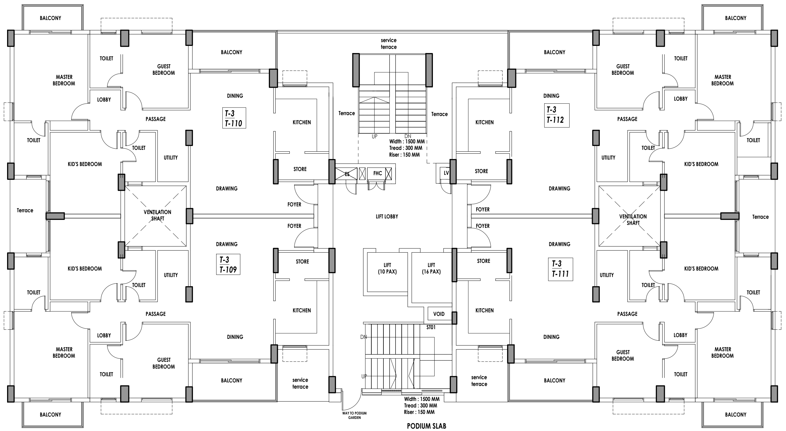
1ST FLOOR PLAN (TYPE-2A TOWER NO. - T-03)
