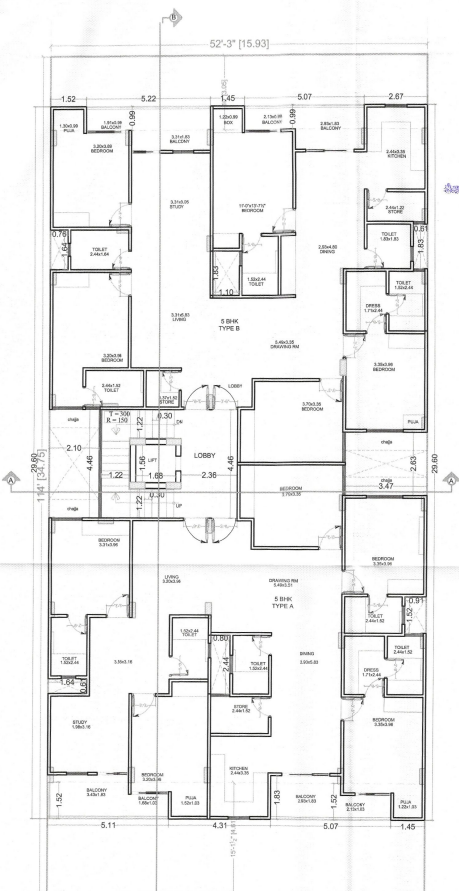
TYPICAL FLR PLAN (GR TO 5TH)
