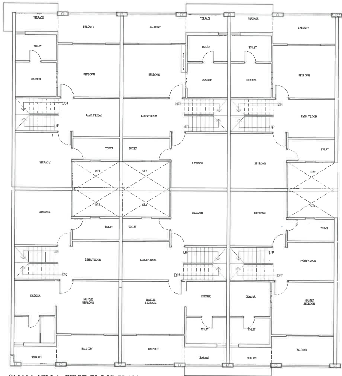
SMALL VILLA -FIRST FLOOR PLAN
