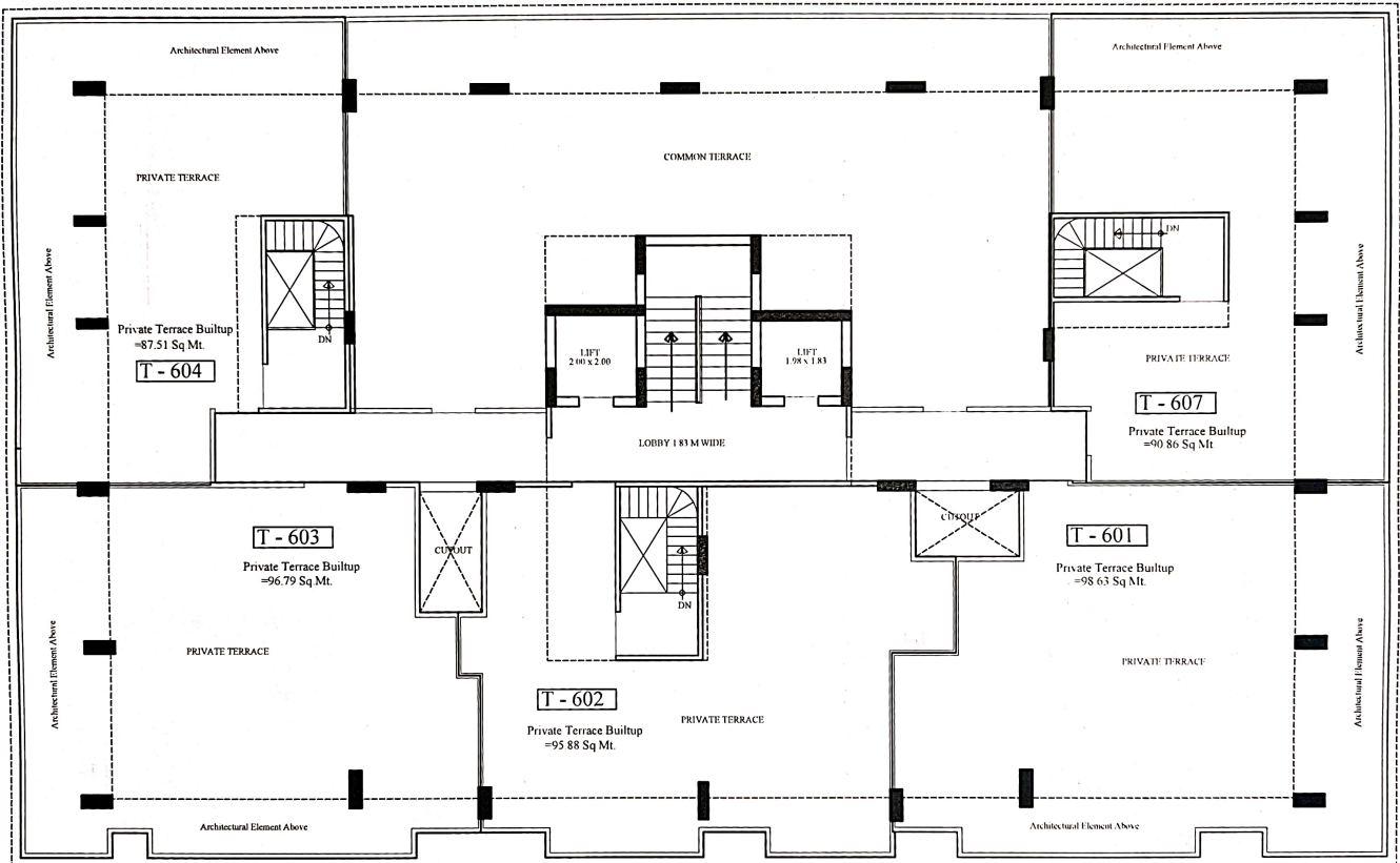
TERRACE PLAN
