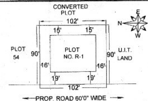
SITE PLAN SCALE 1" = 48'0"
