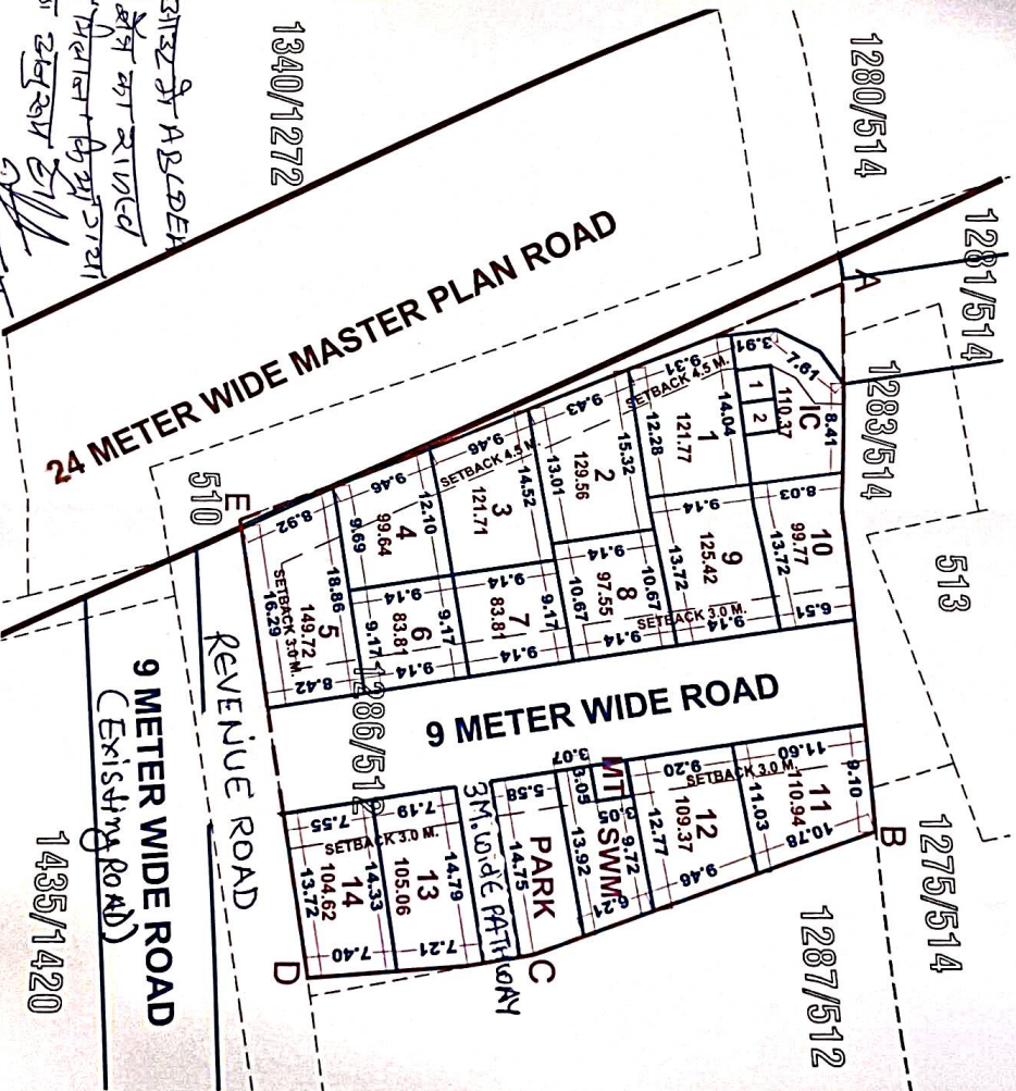
LAYOUT PLAN KHASRA IMPOSE (Scale 1:500)
