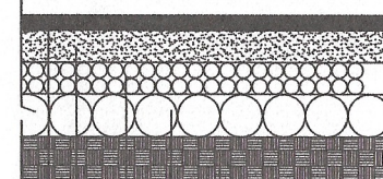
ROAD CRUST SECTION FOR INTERLOCKING TILES
