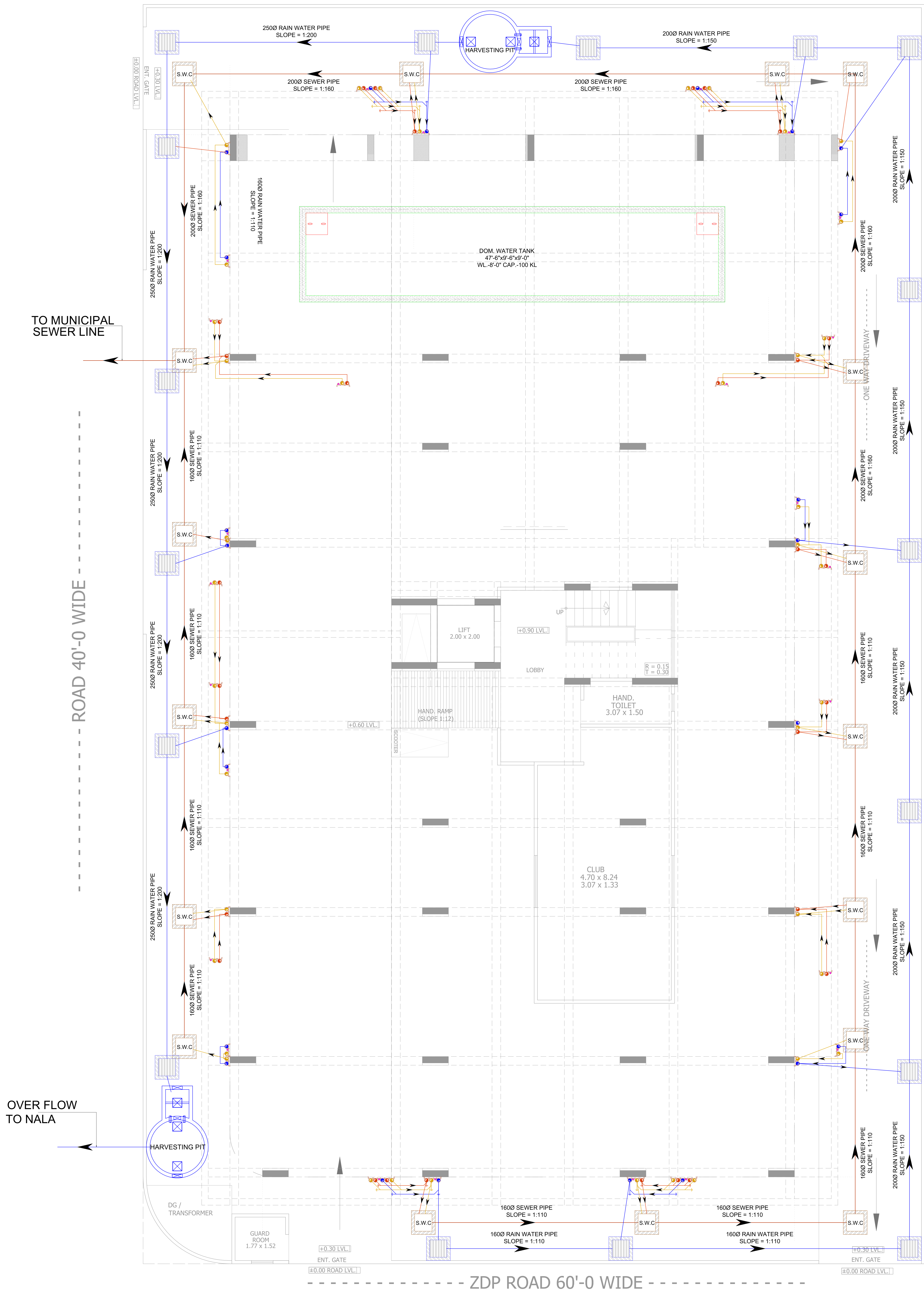
STILT FLOOR RAIN WATER HARVESTING COMMON WATER PIPE ROUTE PLAN
