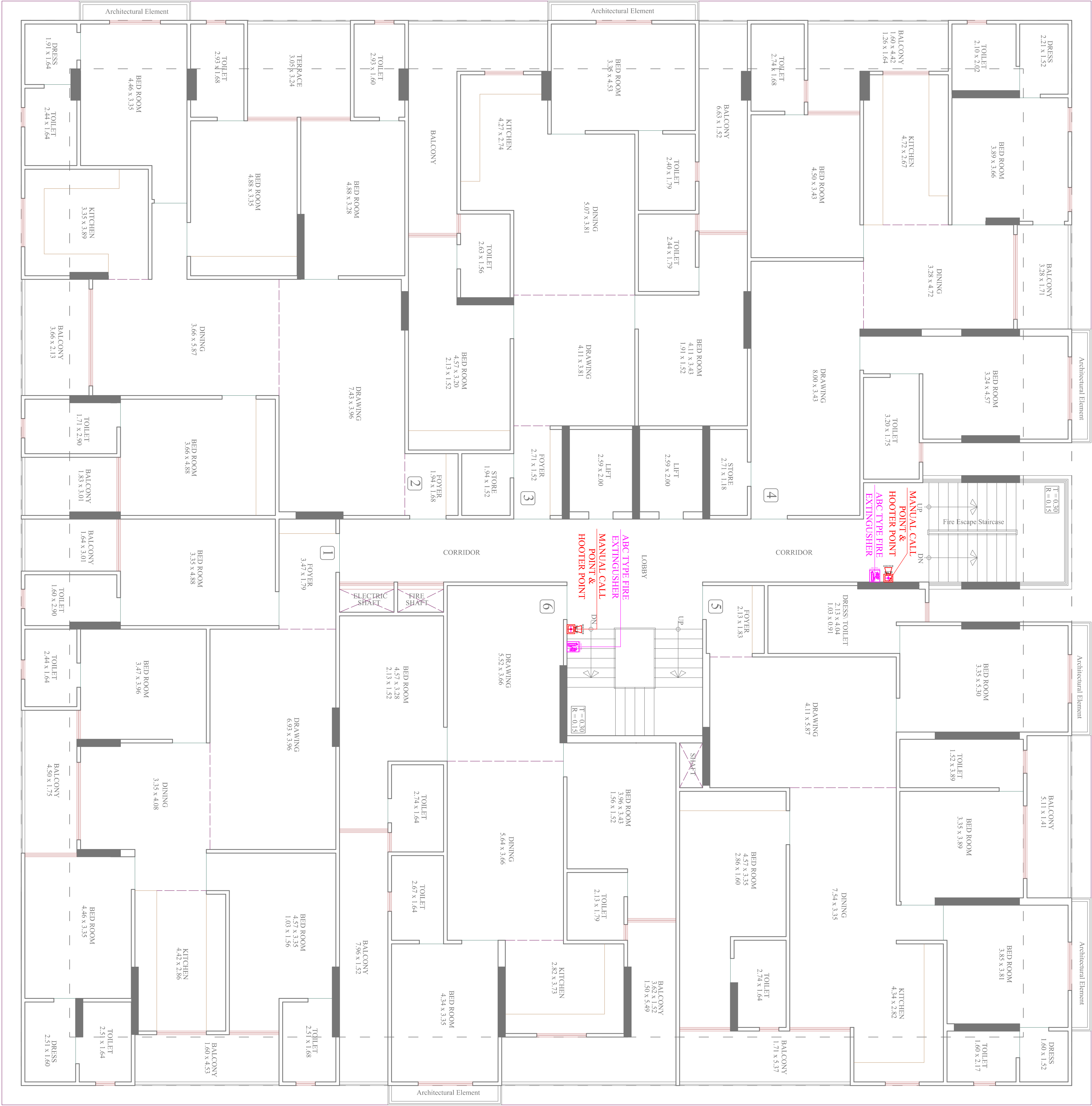
TYPICAL FLOOR PLAN (1st to 11th)
