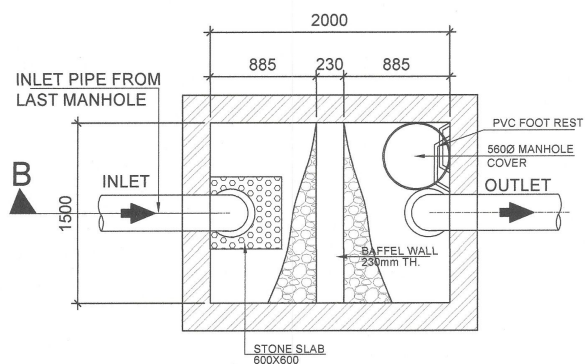
PLAN OF DESILTING CHAMBER & RWH PIT
