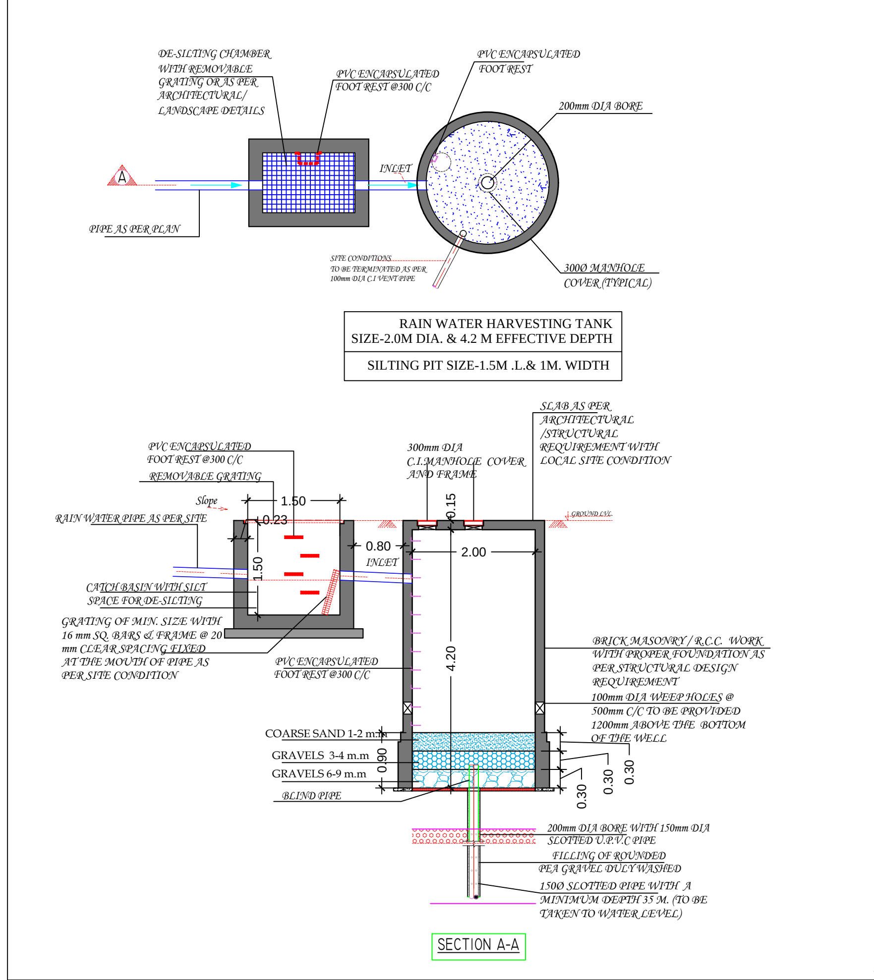
RAIN WATER HARVESTING TANK DETAIL
