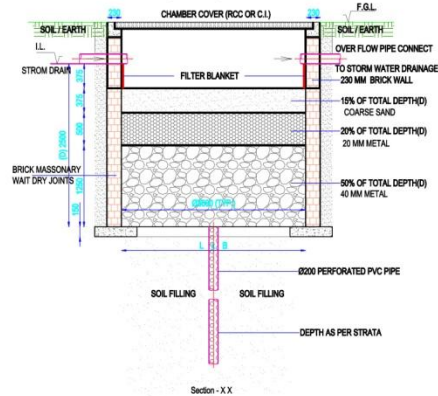
PERCOLATION WELL SECTION (TYPICAL)
