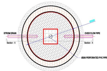
PERCOLATION WELL PLAN (TYPICAL)
