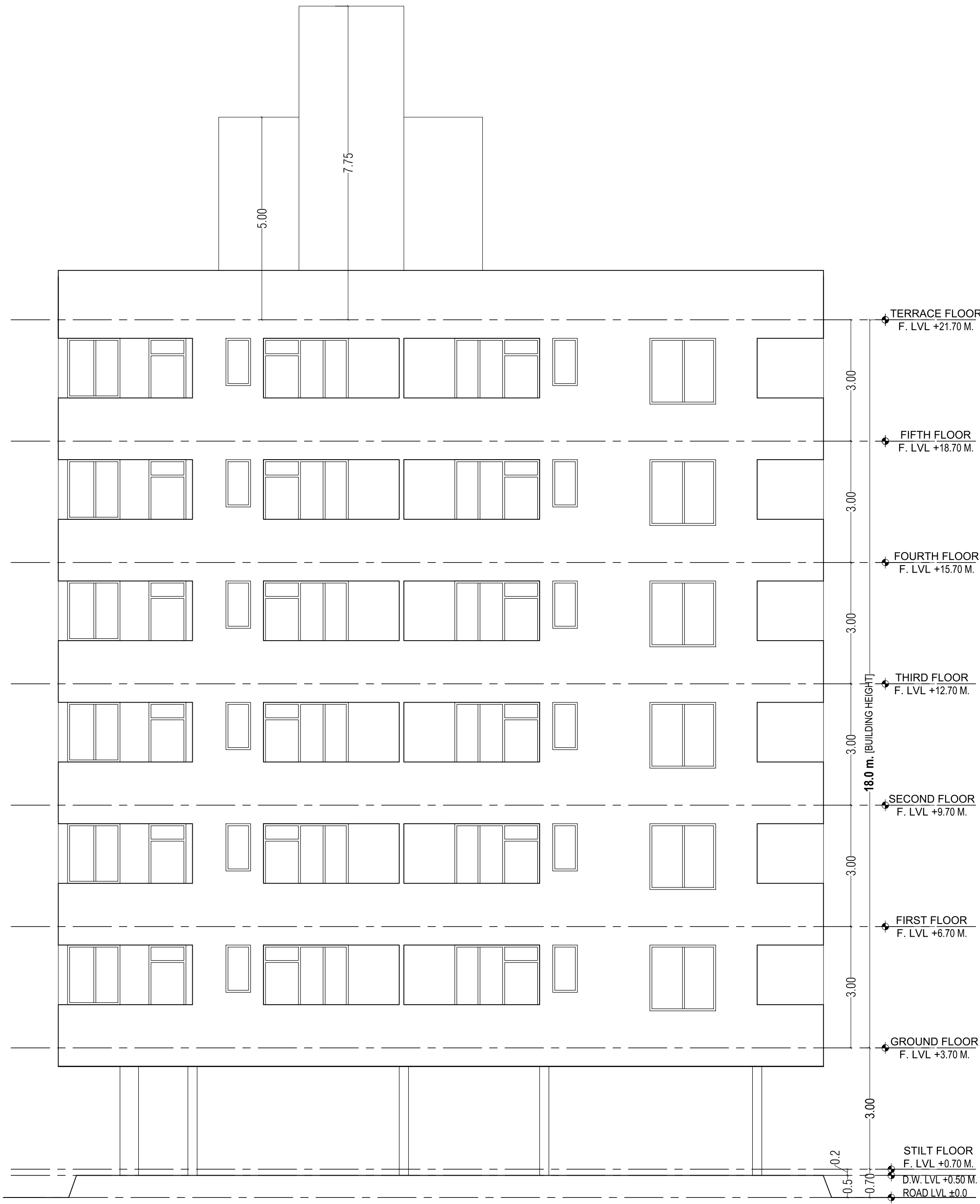
LEFT SIDE ELEVATION
