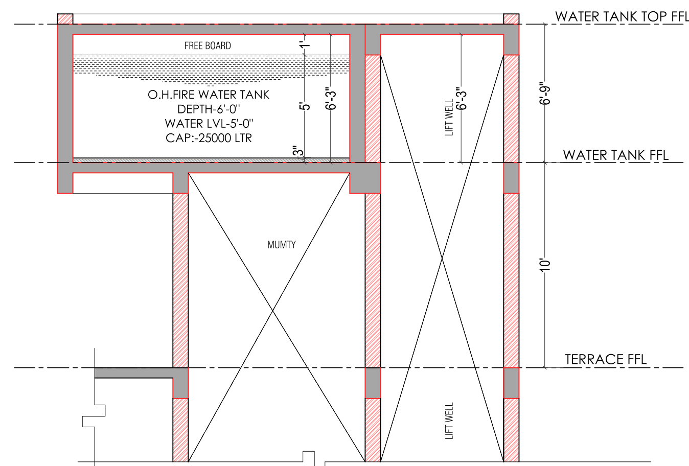
SECTION AT 'A'
