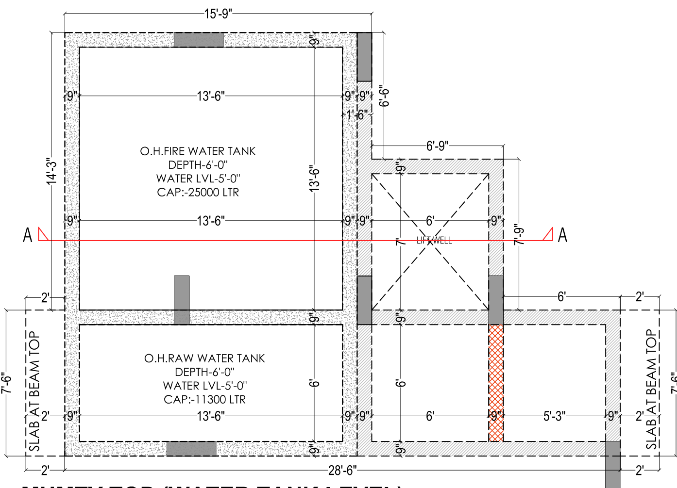
MUMTY TOP (WATER TANK LEVEL) FRAMING PLAN (MAIN STAIRCASE)
