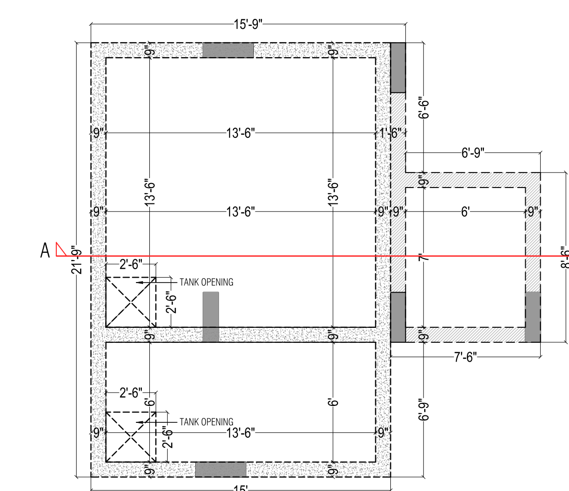
WATER TANK TOP LEVEL FRAMING PLAN (MAIN STAIRCASE)
