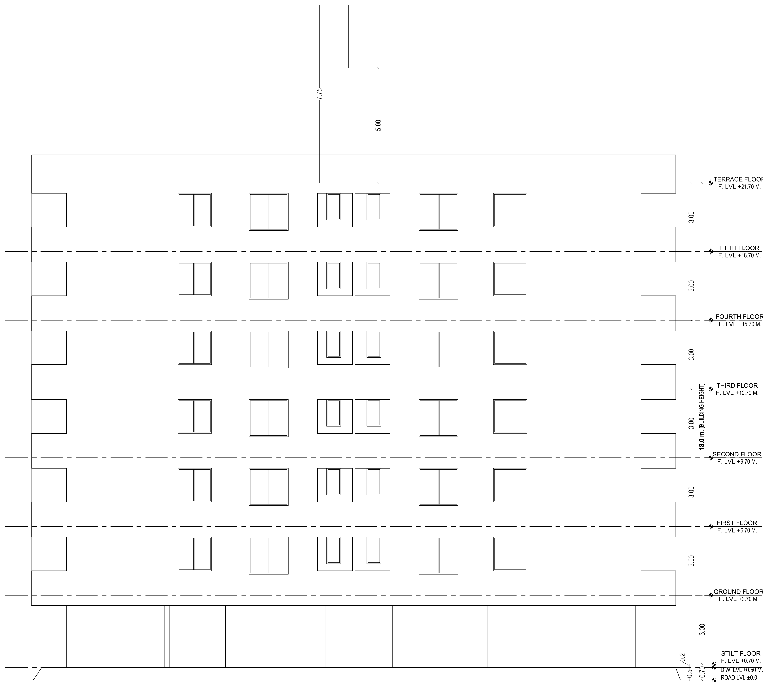
REAR SIDE ELEVATION
