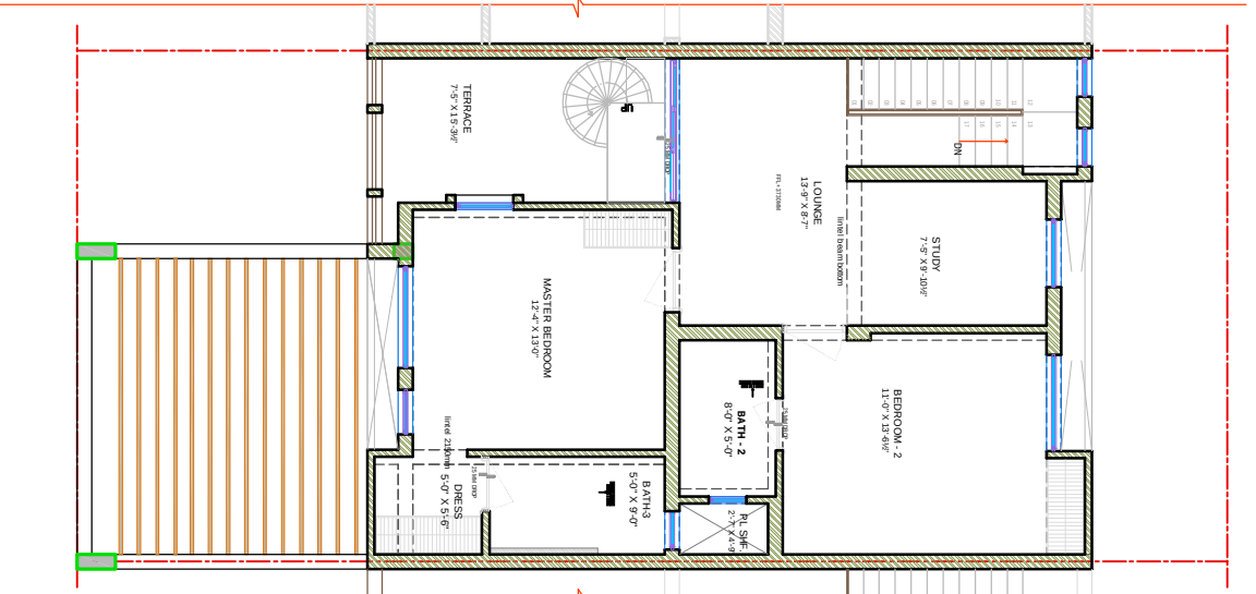
FIRST FLOOR PLAN CARPET AREA : 739.09 SQ.FT. SHAFT AREA - 11.85 SQ.FT. F.F. TERRACE AREA - 109.55 SQ.FT.
