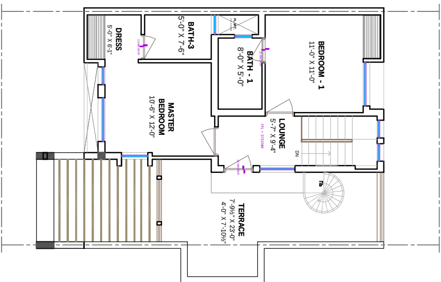
FIRST FLOOR PLAN CARPET AREA : 494.30 SQ.FT.
