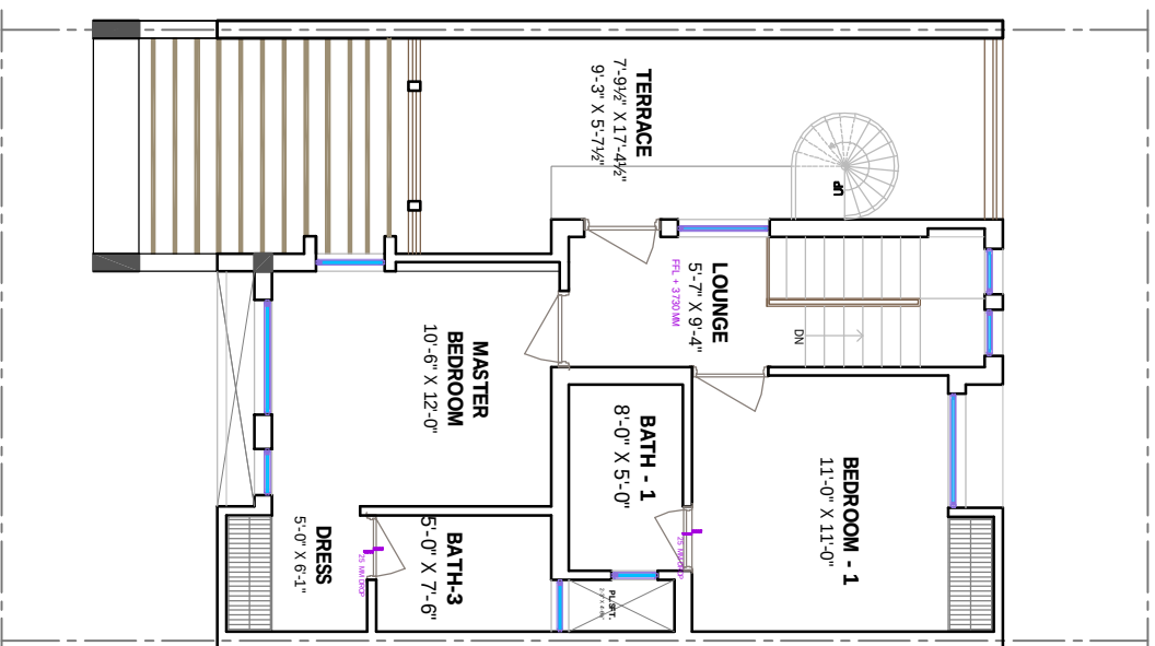
FIRST FLOOR PLAN CARPET AREA : 494.30 SQ.FT.
