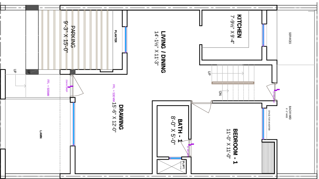
GROUND FLOOR PLAN CARPET AREA : 667.30 SQ.FT.
